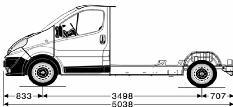
Vivaro FloorCab
